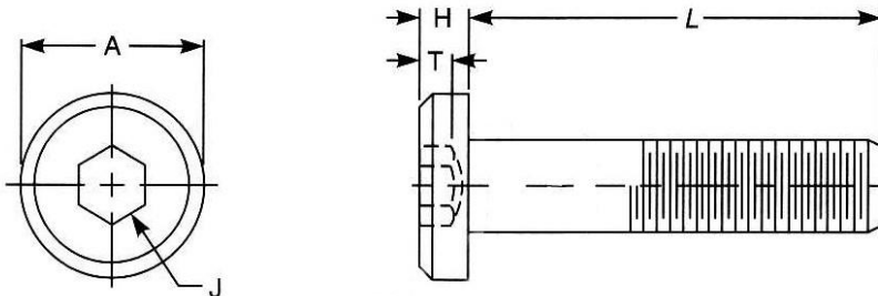
Dimensional Data
