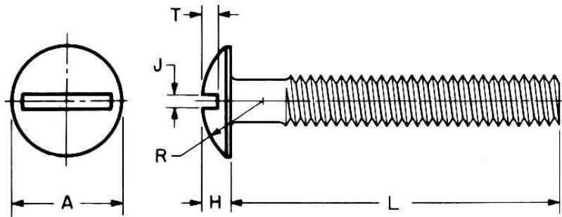
Dimensional Data
